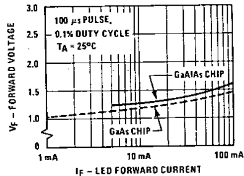
FIGURE 2 Forward Voltage Versus LED Forward Current
